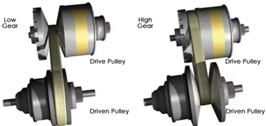
Fig. 13.9 Metal belt CVT ( www.quora.com )
