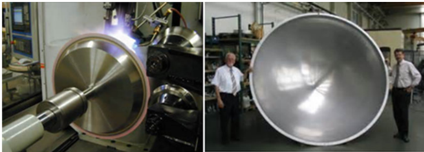
Fig. 14.9 Spinning process and products ( https://www.thomasnet.com )
