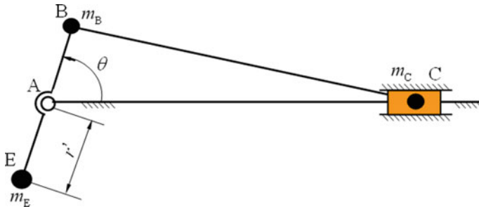
Fig. 7.19 Partial balancing of shaking force of slider-crank mechanism
