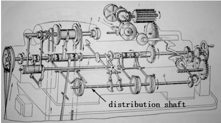
Fig. 7.10 A20 single-spindle automatic turret lathe
