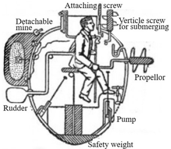
Fig. 4.19 The first submarine “Turtle” ( http://ericshandfield.com/2011/09/observations-bathysphere/ )
