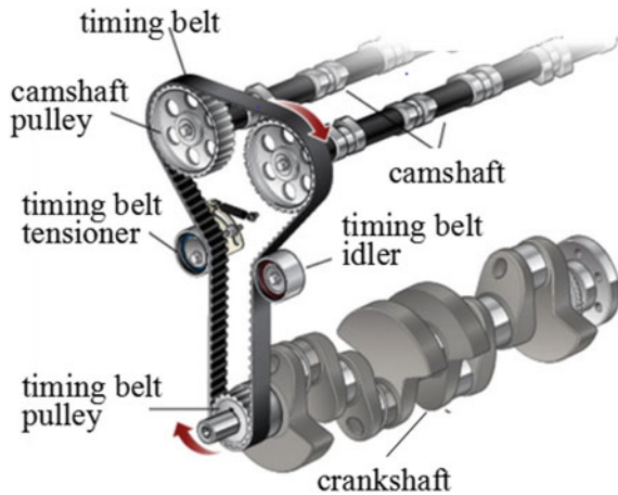
Fig. 13.11 Timing belt used in an engine (from www.repairpal.com )
